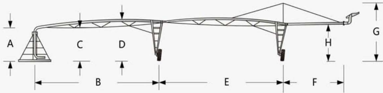
Pivot Span Configuration
