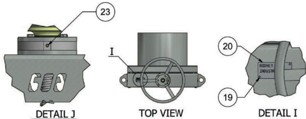
DETAIL J
